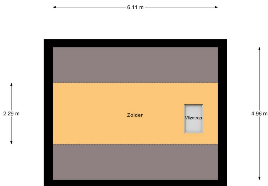
Garage Zolder
